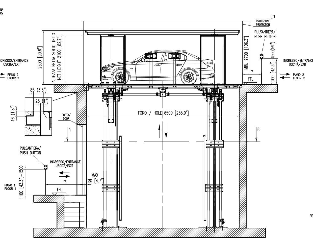
VISTA FRONTALE HYPERLIFT ALZATO - HYPERLIFT LIFTED FRONT VIEW
