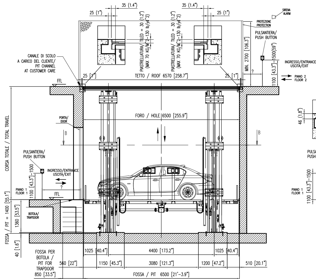
VISTA FRONTALE HYPERLIFT ABASSATO - HYPERLIFT COLLAPSED FRONT VIEW
